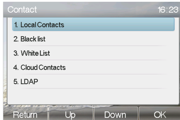
Figure 25 - Phonebook screen
